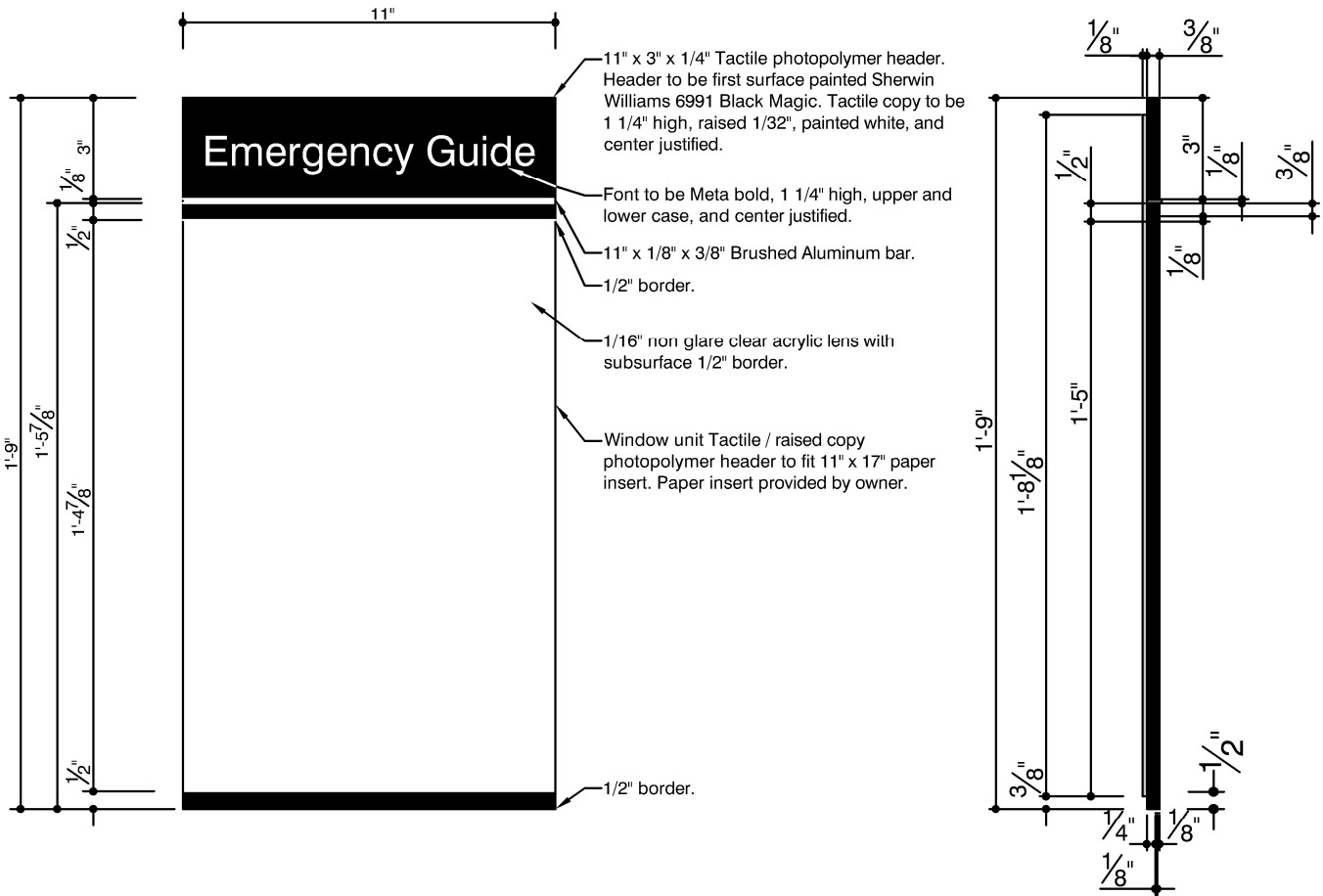
FRONT ELEVATION
